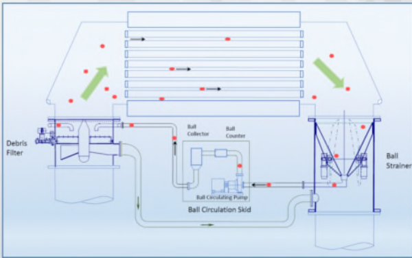
Typical PID representation of a condenser installation with Debris Filter and CTCS
